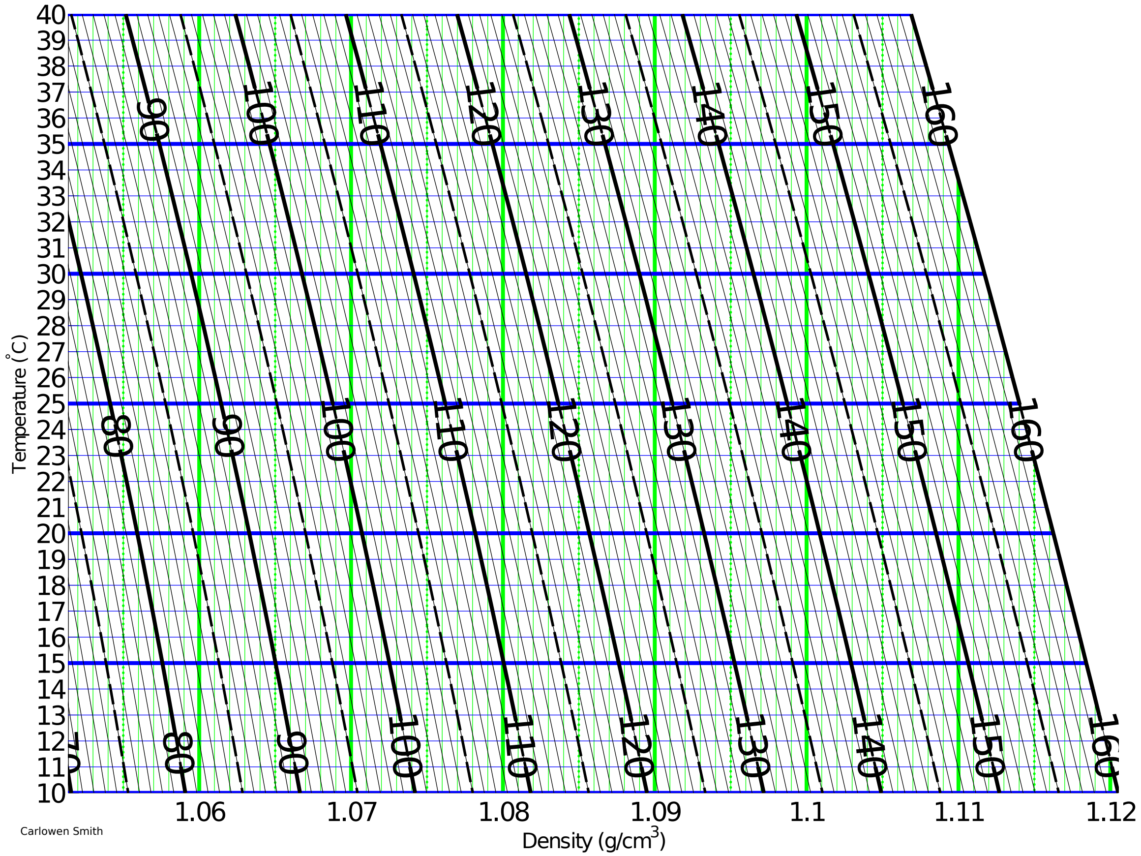
Salt Fraction (ppt) required for a given Density from Ruddick and Shirtcliffe (1979)
